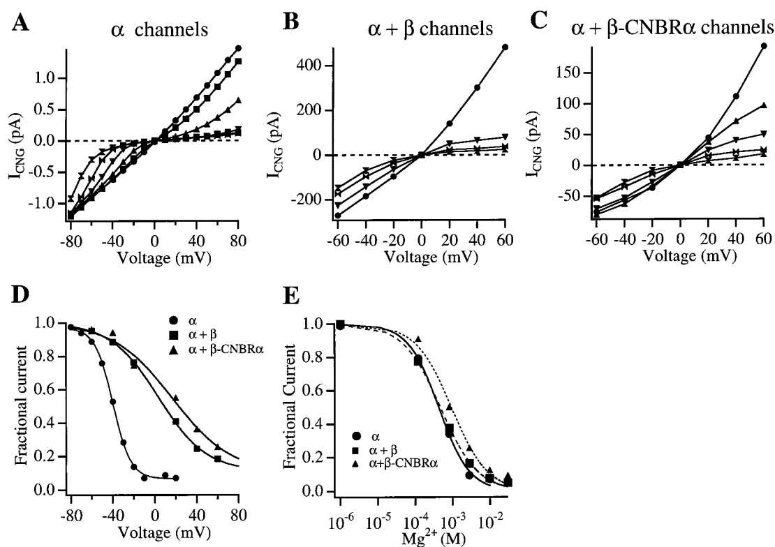
FIGURE 7 Block by internal Mg^{2+} . Current-voltage curves for a patch with \alpha channels ( A ), \alpha + \beta channels ( B ), or \alpha + \beta -CNBR \alpha channels ( C ) in the absence or presence of a range of internal Mg^{2+} concentrations. For all three panels, the Mg^{2+} concentrations are: (circles) 0, (squares) 120 \mu M, (triangles) 811 \mu M, (inverted triangles) 2.81 mM, (bows) 9.81 mM, (inverted bows) 29.8 mM. In ( A ), the data are the steady-state currents from a family of potentials from -80 mV to 80 mV at each Mg^{2+} concentration. Because of desensitization, the data in ( B ) and ( C ) were obtained by applying pseudo-ramps at each concentration, at 1/s . Each pseudo-ramp was a series of 30-ms steps progressing from -60 mV to 60 mV in 20-mV steps, and each measurement was made at the end of each step. Thus, any errors due to desensitization should be comparable to those using our usual pulse protocol (Fig. 1, inset ). ( D ) Normalized current-voltage relations for \alpha channels, \alpha + \beta channels, and \alpha + \beta -CNBR \alpha channels at a fixed Mg^{2+} concentration of 2.81 mM. Superimposed on the data are fitted Boltzmann relations of the form I = (I_{max} - I_s)/(1 + \exp[z\delta(V - V_{1/2})/kT]) + I_s , where V_{1/2} is the voltage at which the current is half-blocked, z is the valence of the blocker (2 for Mg^{2+} ), \delta is the fraction of the transmembrane electrical field sensed by the blocker, I_s is the current remaining at very positive potentials, and I_{max} , R , and T have their usual meaning. For \alpha channels, z\delta = 2.8e^- and V_{1/2} = -56 mV; for \alpha + \beta channels, z\delta = 1.1e^- and V_{1/2} = 3 mV; for \alpha + \beta -CNBR \alpha channels, z\delta = 0.90e^- and V_{1/2} = 17 mV. ( E ) Normalized dose-response relations for Mg^{2+} block of the three types of channels at a fixed potential of 60 mV. Superimposed on the data are fitted Hill equation curves of the form I = I_{max}K_{1/2}^n/(K_{1/2}^n + [Mg^{2+}]^n) , where I is the steady-state current, K_{1/2} is the concentration of Mg^{2+} that produces half-block, and n is the Hill coefficient. We constrained I_{max} to be unity. For \alpha channels, K_{1/2} = 425 \mu M and n = 1.06 . For \alpha + \beta channels, K_{1/2} = 469 \mu M and n = 0.88 . For \alpha + \beta -CNBR \alpha channels, K_{1/2} = 927 \mu M and n = 0.91 .
